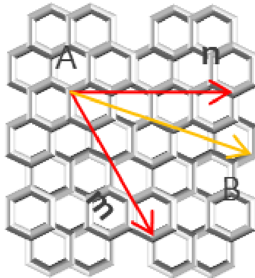
Figure 1. 2 m , n indices to describe the electrical nature of carbon nanotubes. Take the origin carbon as the number 1 carbon, draw vector a_1 to atom 3 and draw vector a_2 to atom 5. Coming from A to B, the number of atoms coming in a_1 and a_2 directions are m and n .
